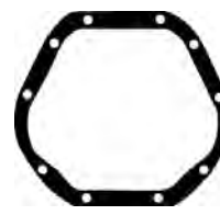
P27768T P27768TC 10 Holes 10 Troues 10 Orificios 9-5/16" x 10-5/16"
