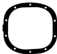
P27872 10 Holes 10 Troux 10 Orificios 10-9/16" x 9-9/16"
