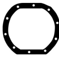
P27139TC 10 Holes 10 Troux 10 Orificios 9-11/16" x 10-7/8"
