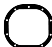
P38154TC 10 Holes 10 Troues 10 Orificios 9-7/8" x 10-7/8"
