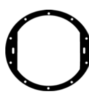
P27857 P27857TC 10 Holes 10 Troues 10 Orificios 11" x 10-1/4"
