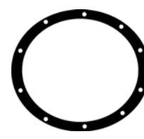
P27801 10 Holes 10 Troux 10 Orificios 9-1/4" x 10-3/8"
