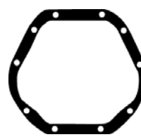
P27768T P27768TC 10 Holes 10 Troux 10 Orificios 10-7/16" x 9-3/8"
