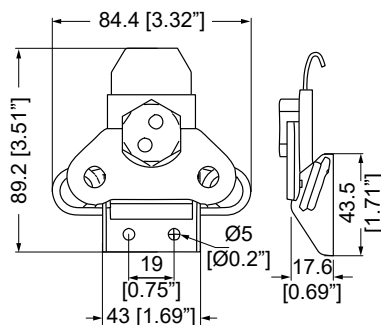
7566 Large surface mount twist latch. Spring-loaded.
