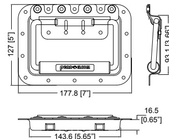
H7165 Rivet Protected Recessed Handle with Extended Grip. Double Sprung. Use Backplate H1905.
