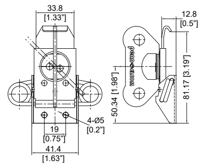
7568 Large low level surface mount twist latch. Spring-loaded.
