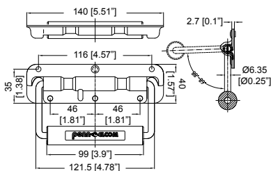
H1053 Surface Mount Spring-Loaded Handle with 3/4" (19mm) rubber Grip.
