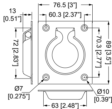
5715 Recessed Tie Down/Ring Pull.
