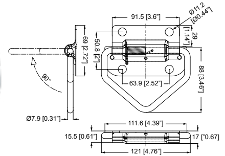
2467 Surface Mount Spring-Loaded Tie Down Anchor.
