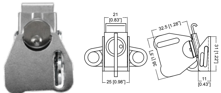
7339 Small surface mount twist latch. Padlockable.
