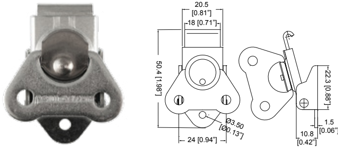
7335 Small low level surface mount twist latch with exposed mounting hole.
