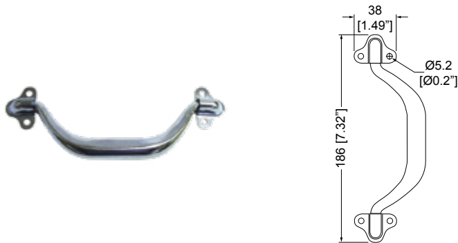
2386 Surface Mount Tubular Handle. Supplied as 3-Piece Kit for Self Assembly.
