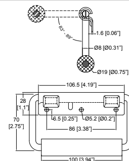
2356 Surface Mount Spring-Loaded Handle with 3/4" (19mm) rubber Grip.
