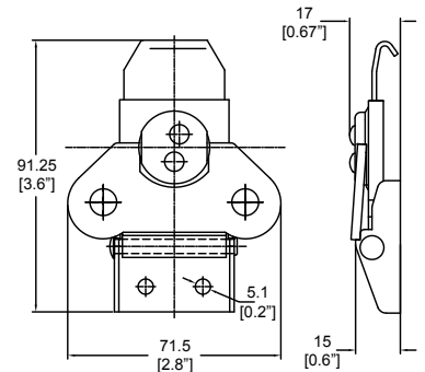
7538 Large Low Level surface mount twist latch.
