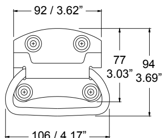
2457 Chest Handle with Countersunk Mounting Holes.
