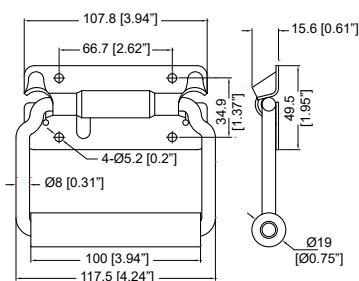
2351 Surface Mount Spring-Loaded Handle with 3/4" (19mm) rubber Grip.
