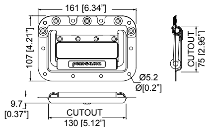
H7159 Heavy Duty Rivet Protected Recessed Handle. Double Sprung. 5/16" (8mm) Bail with 11/16" (17mm) Grip Use Backplate H1906.
