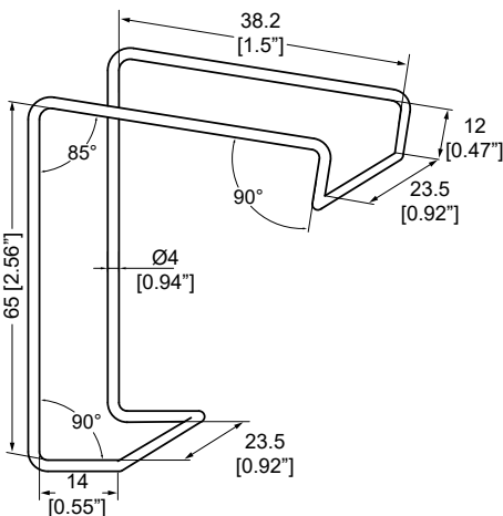
#2 Small Spring lock
