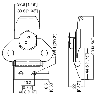
7536 Large surface mount twist latch.
