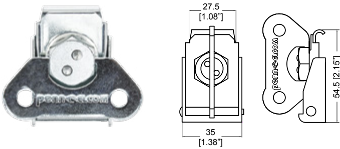
7435 Medium twist latch with 0.16" (4mm) mounting holes.
