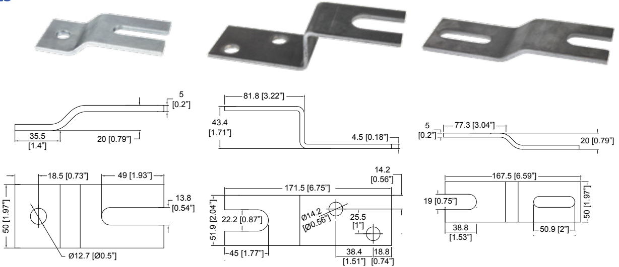
8649 Bent fork bracket with 1 mounting hole
