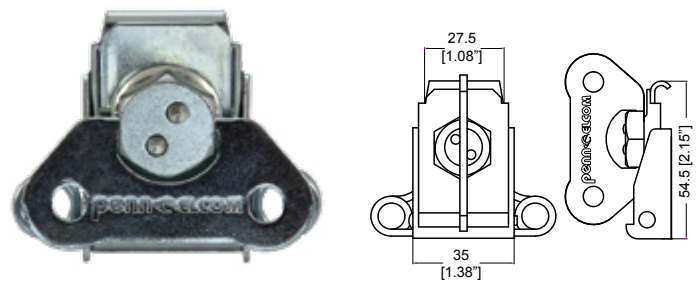
7460 Medium twist latch. Spring loaded.
