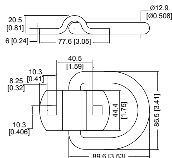
5711 Heavy Duty D-Ring. Use backplate 5711BP.
