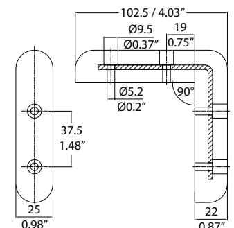
5387GREY Heavy Duty Corner Protector. PVC with Steel Insert.
