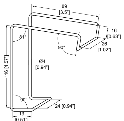
#4 Large Spring lock
