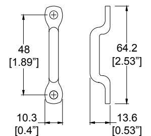
H1435 Snap Back Spring Shackle. Test Certificate available. H1460 Backplate for H1435.
