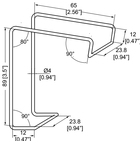
#3 Medium Spring lock
