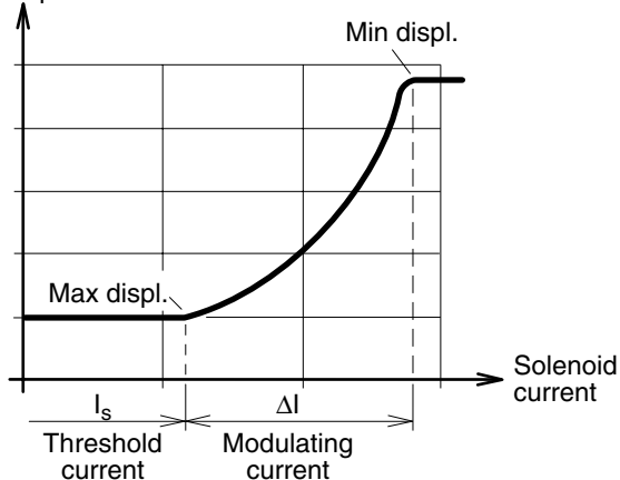
Shaft speed vs. solenoid current (EP control).
