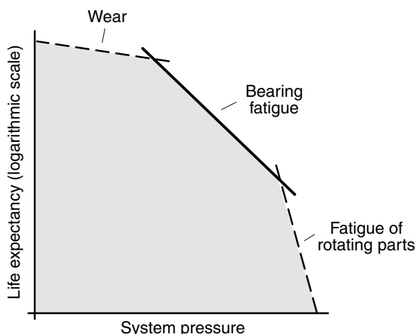
Hydraulic motor life versus system pressure.
