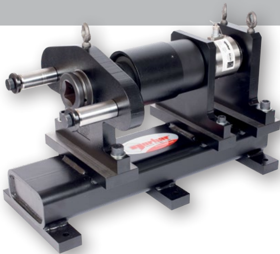
Power Tool Test Rig shown with 1 1/2" M/F Static Transducer (not included)
