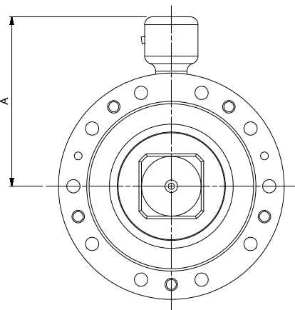
Fixed Connector
