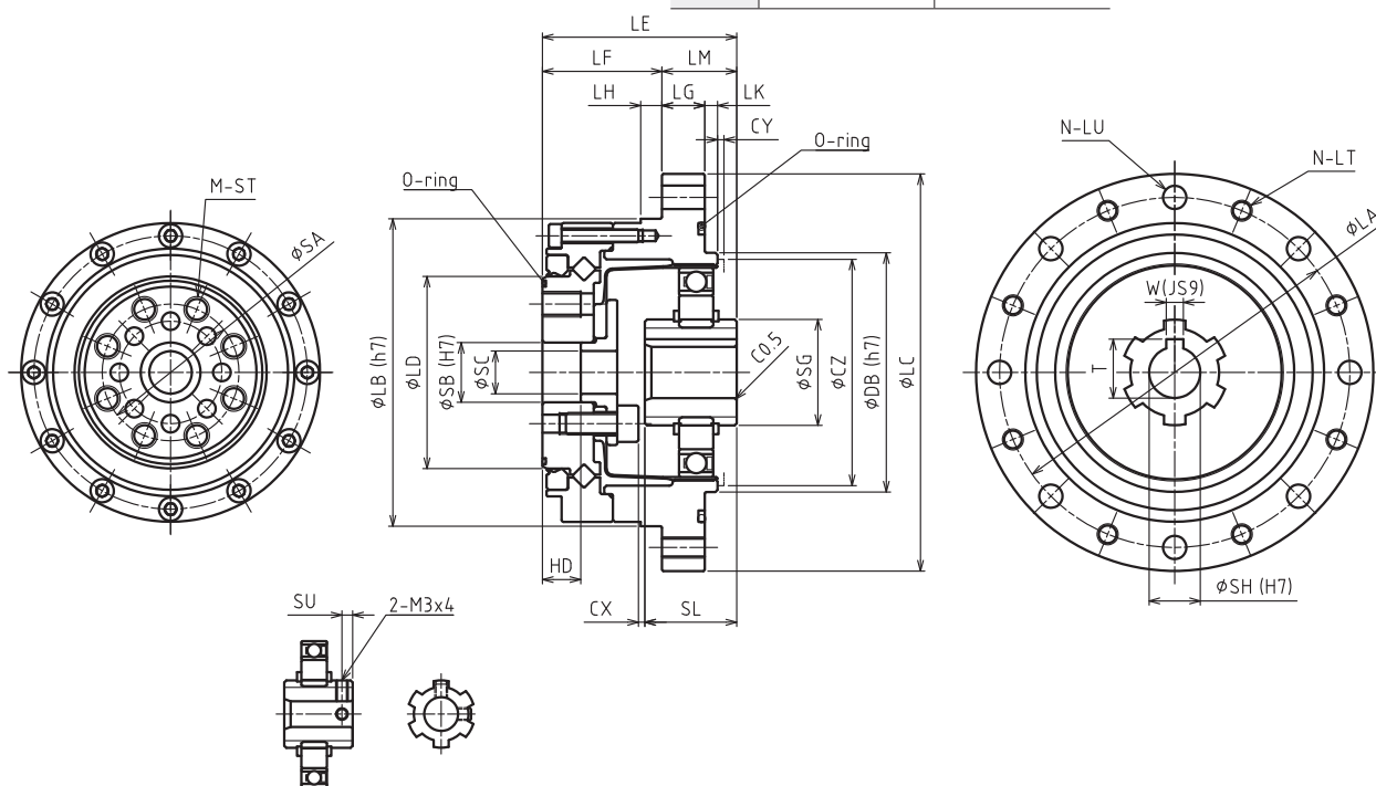
INPUT SHAFT FOR 35&amp;42
