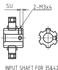
INPUT SHAFT FOR 35&42
