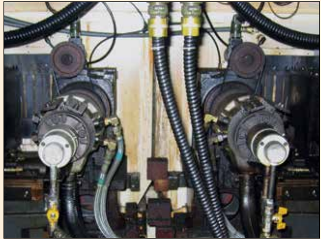
DEUBLIN 2-passge Unions on CNC Turning Center
